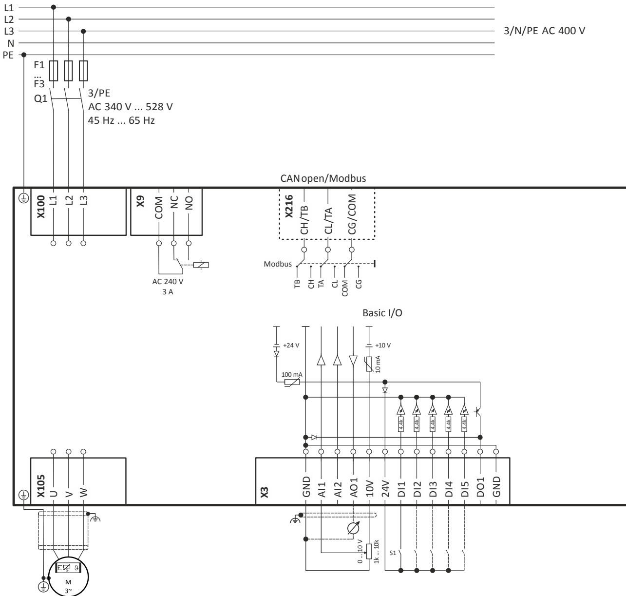
Fig. 5: Wiring example
